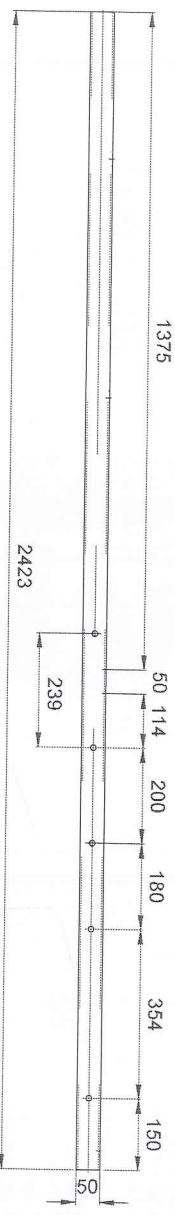
TOP VIEW
